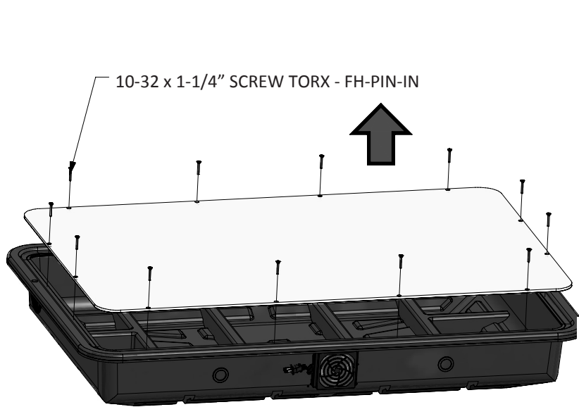
HORIZONTAL DISPLAY SHIELD
