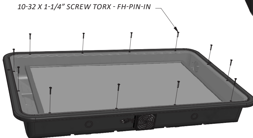
HORIZONTAL DISPLAY SHIELD
